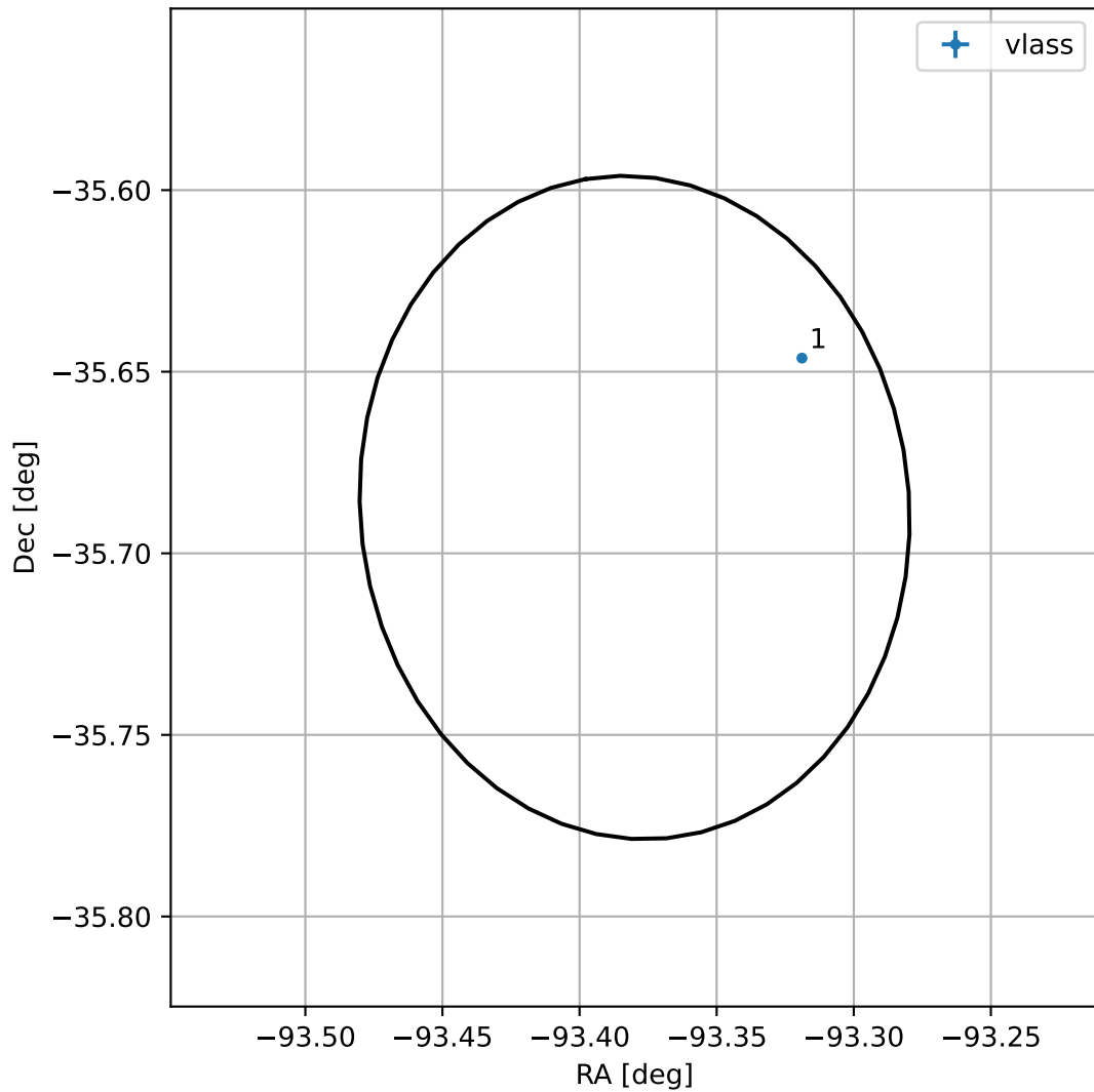
4FGL J1746.4-3541
