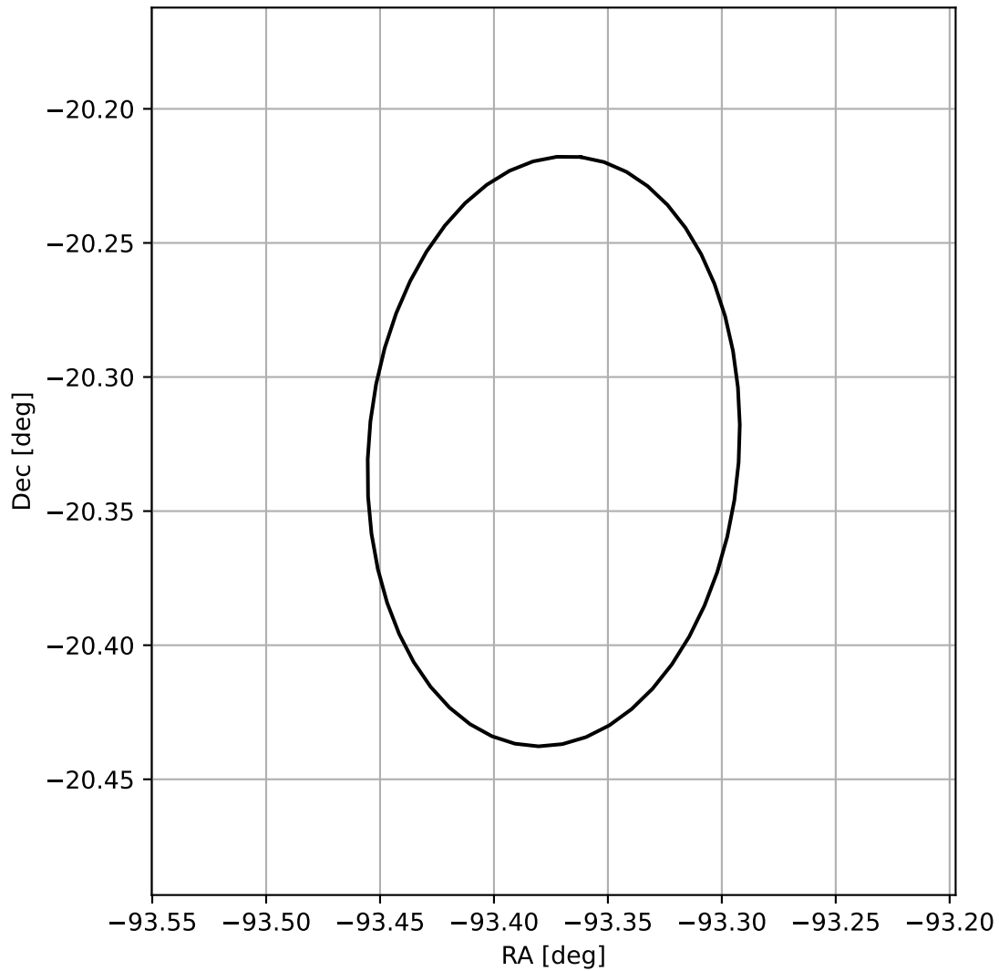
4FGL J1746.5-2019
