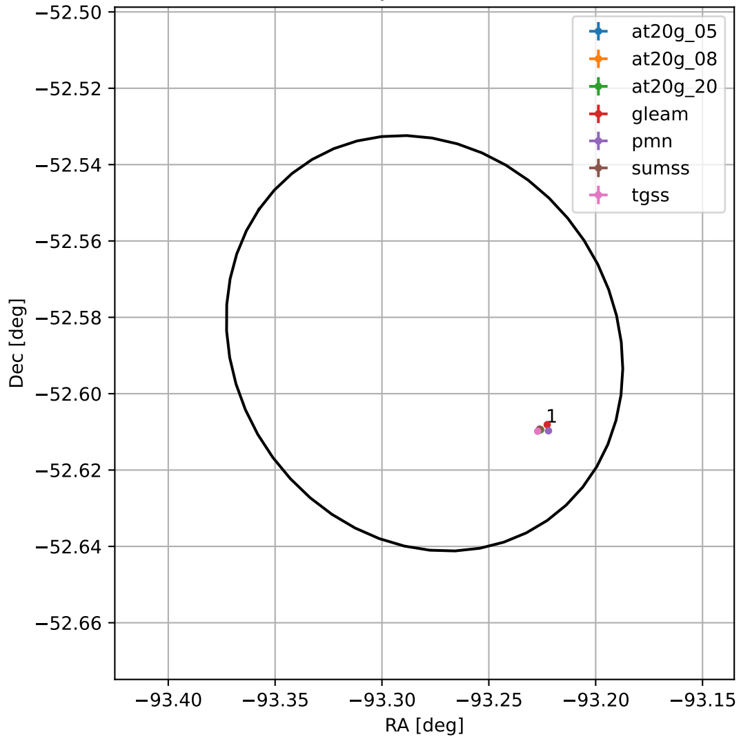
4FGL J1746.8-5235
