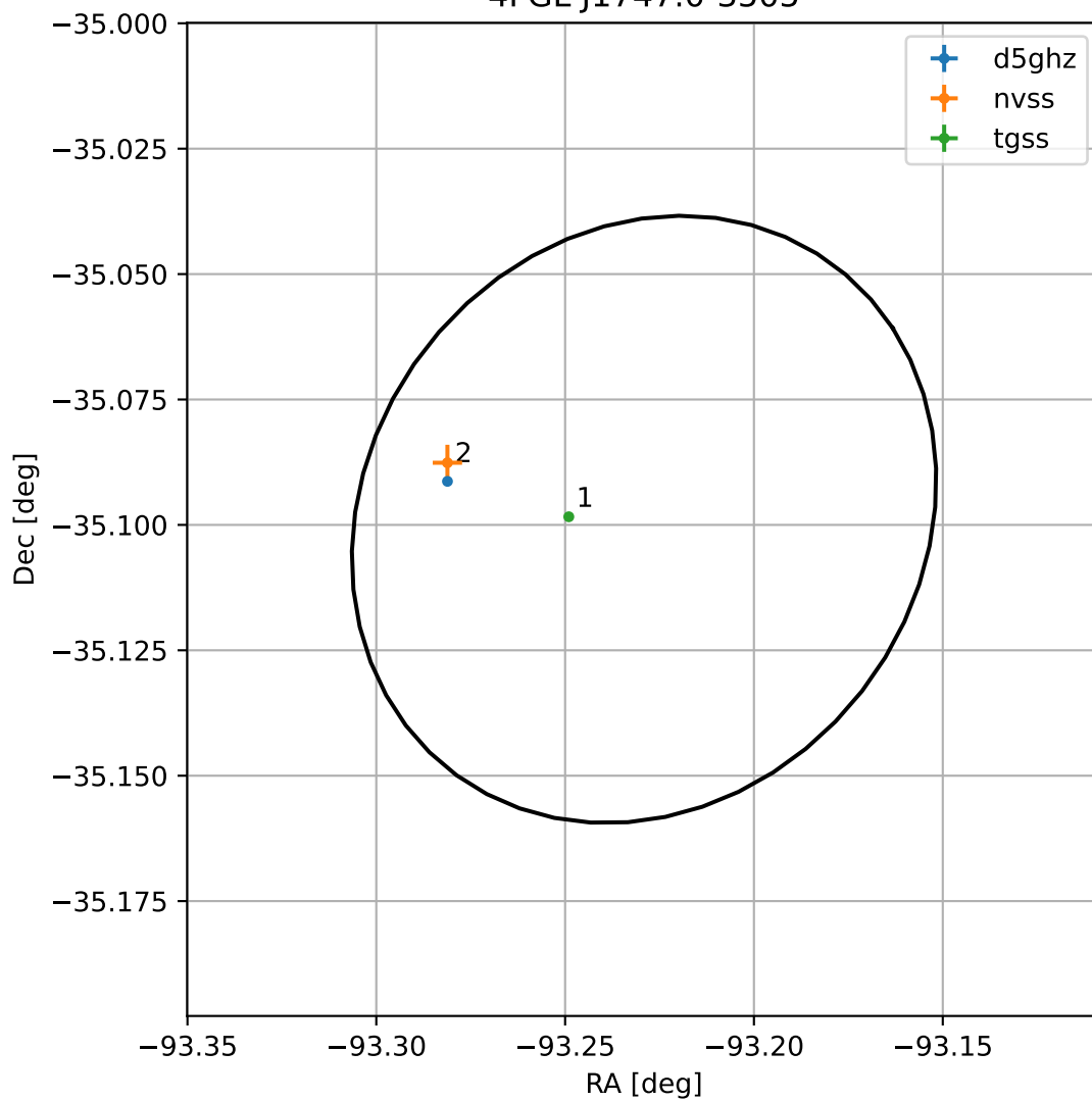
4FGL J1747.0-3505
