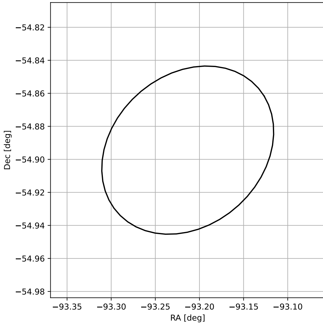
4FGL J1747.1-5453
