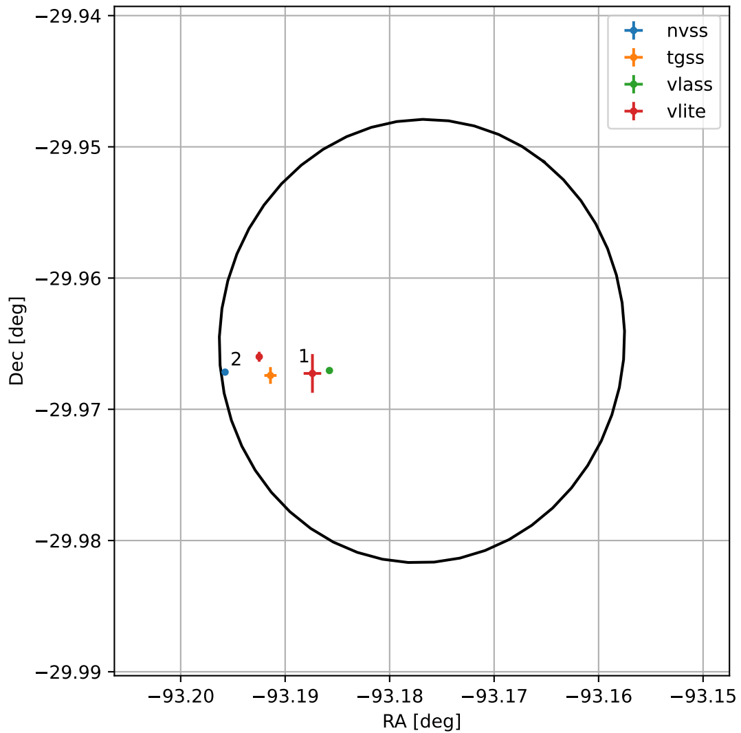
4FGL J1747.2-2957
