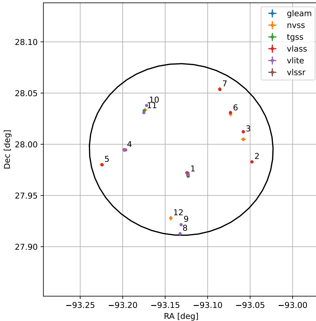
4FGL J1747.4+2759
