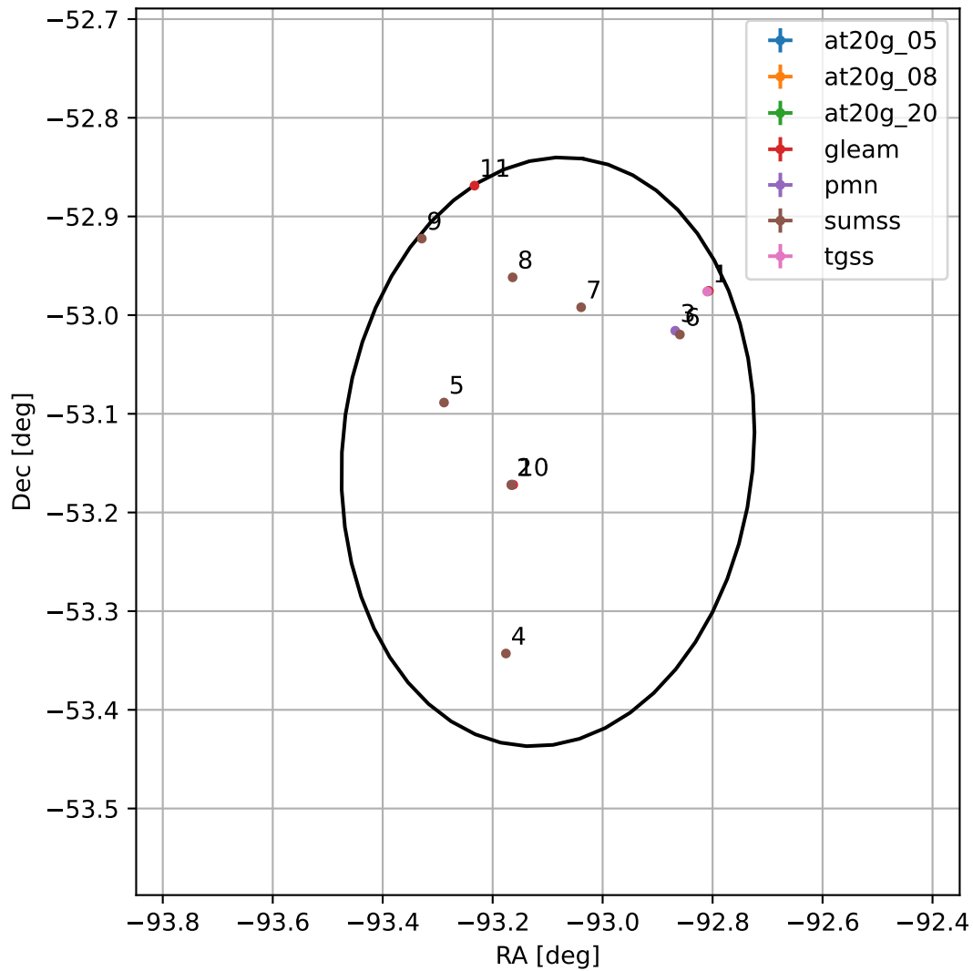
4FGL J1747.6-5308
