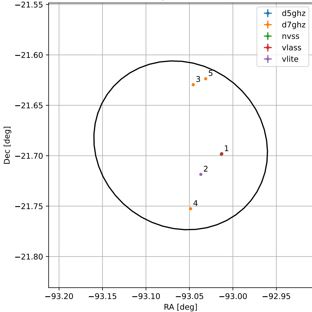
4FGL J1747.7-2141
