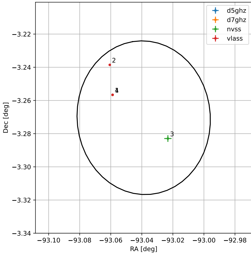
4FGL J1747.8-0316
