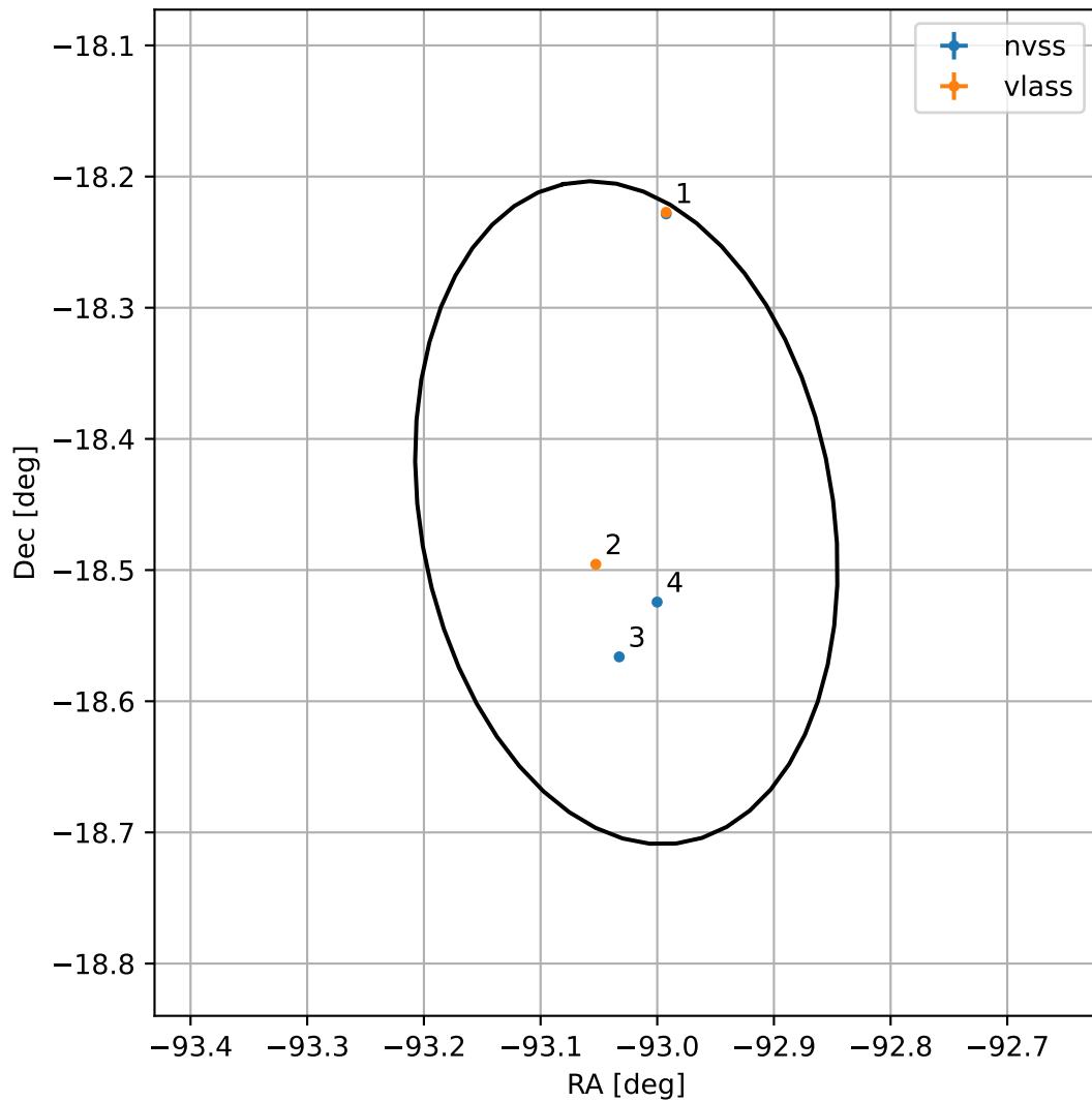
4FGL J1747.8-1827
