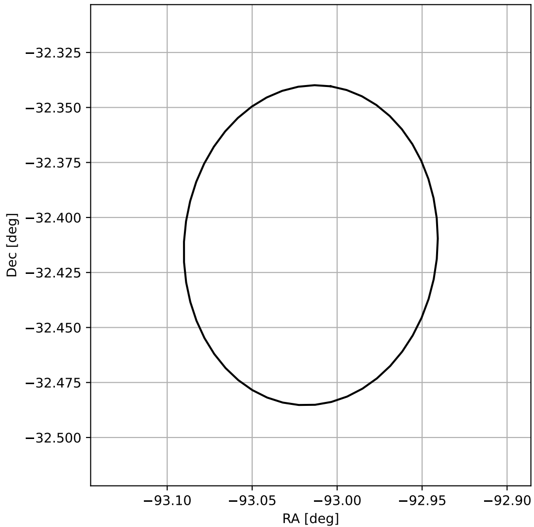
4FGL J1747.9-3224
