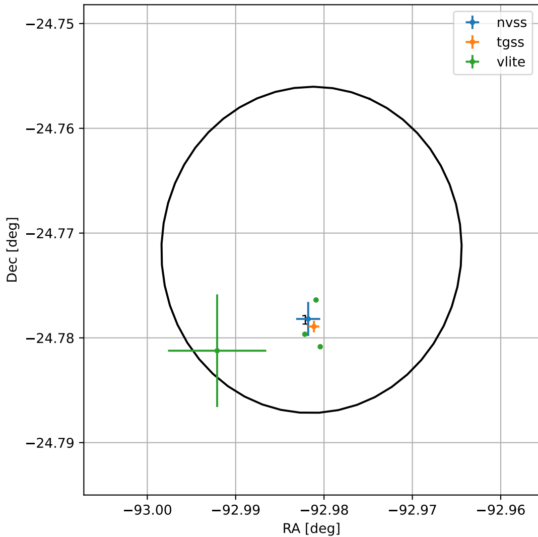
4FGL J1748.0-2446
