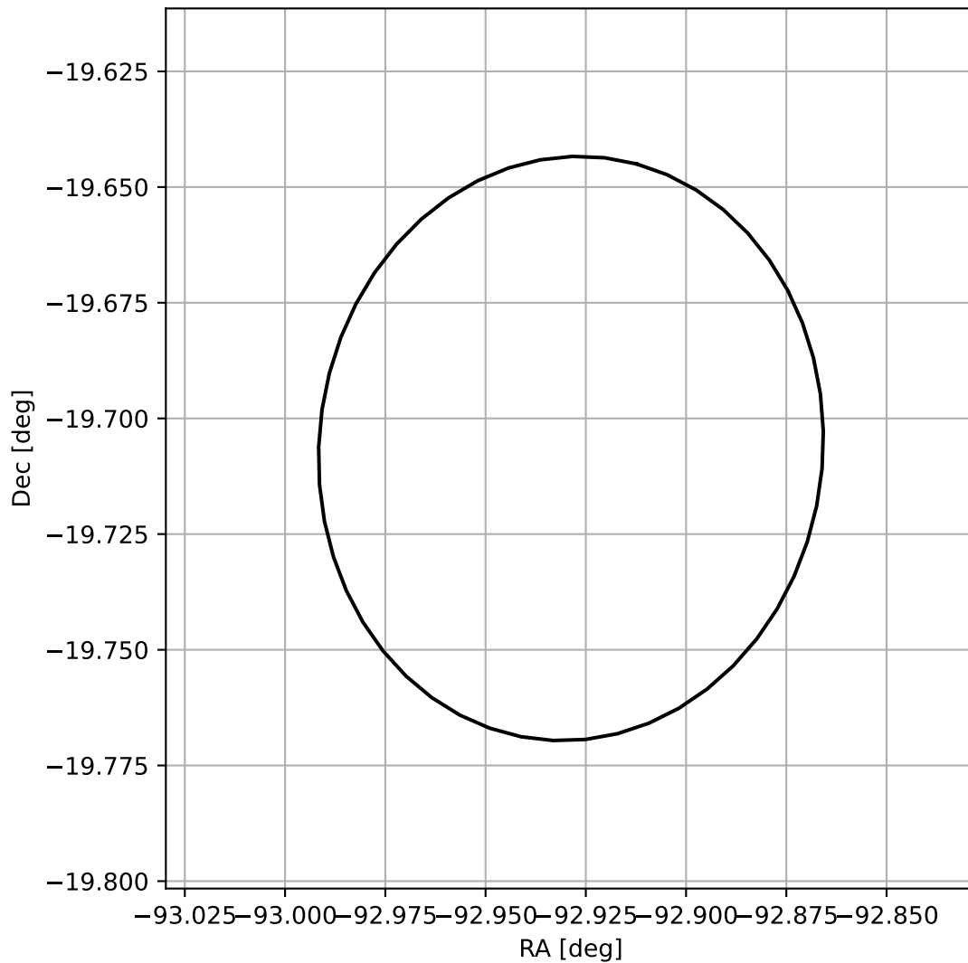
4FGL J1748.2-1942
