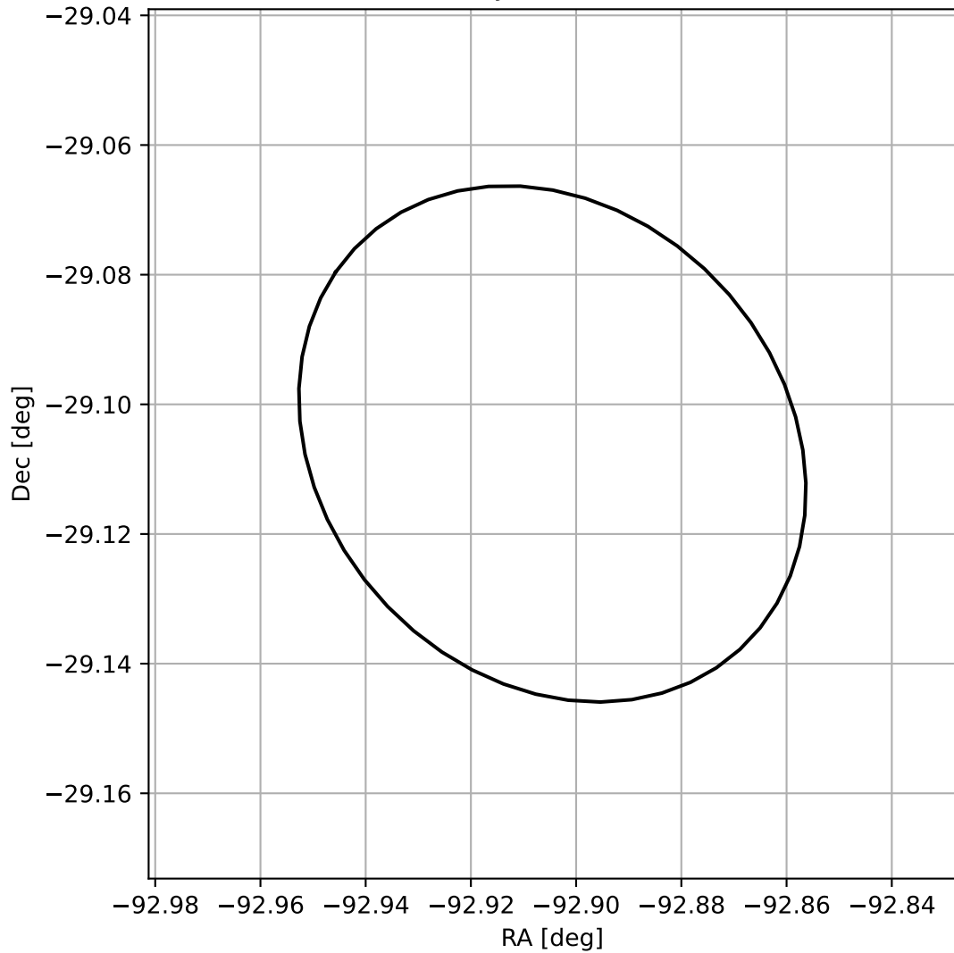
4FGL J1748.3-2906
