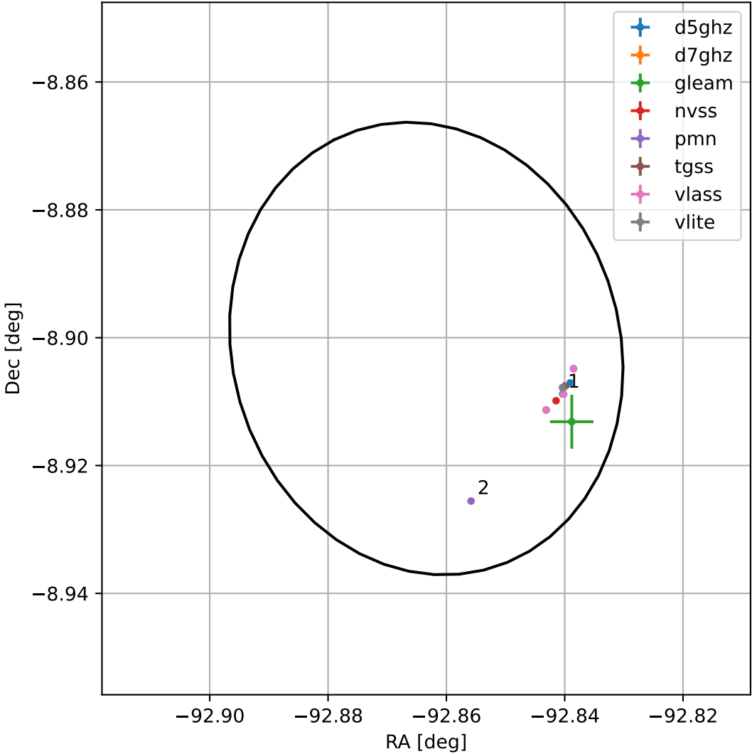
4FGL J1748.5-0854
