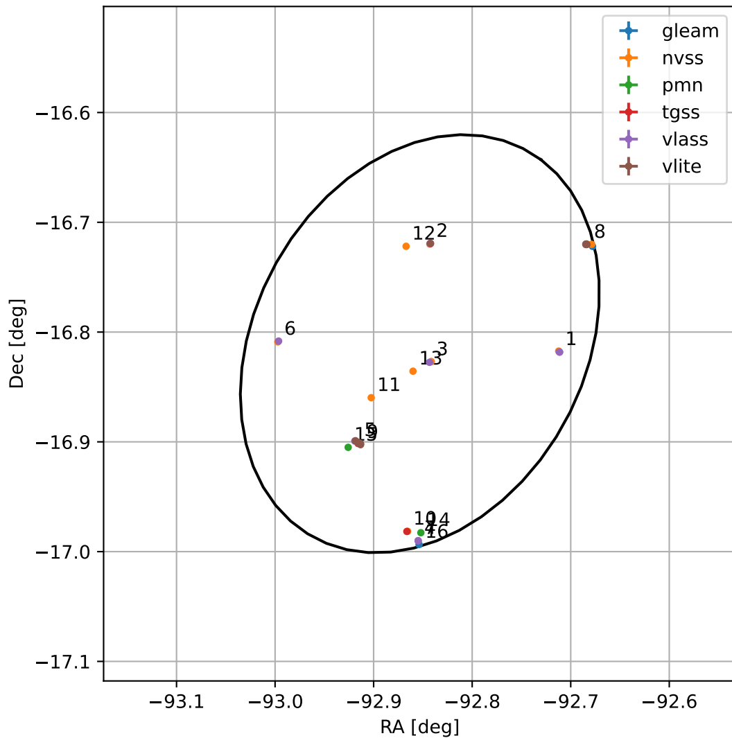
4FGL J1748.5-1648
