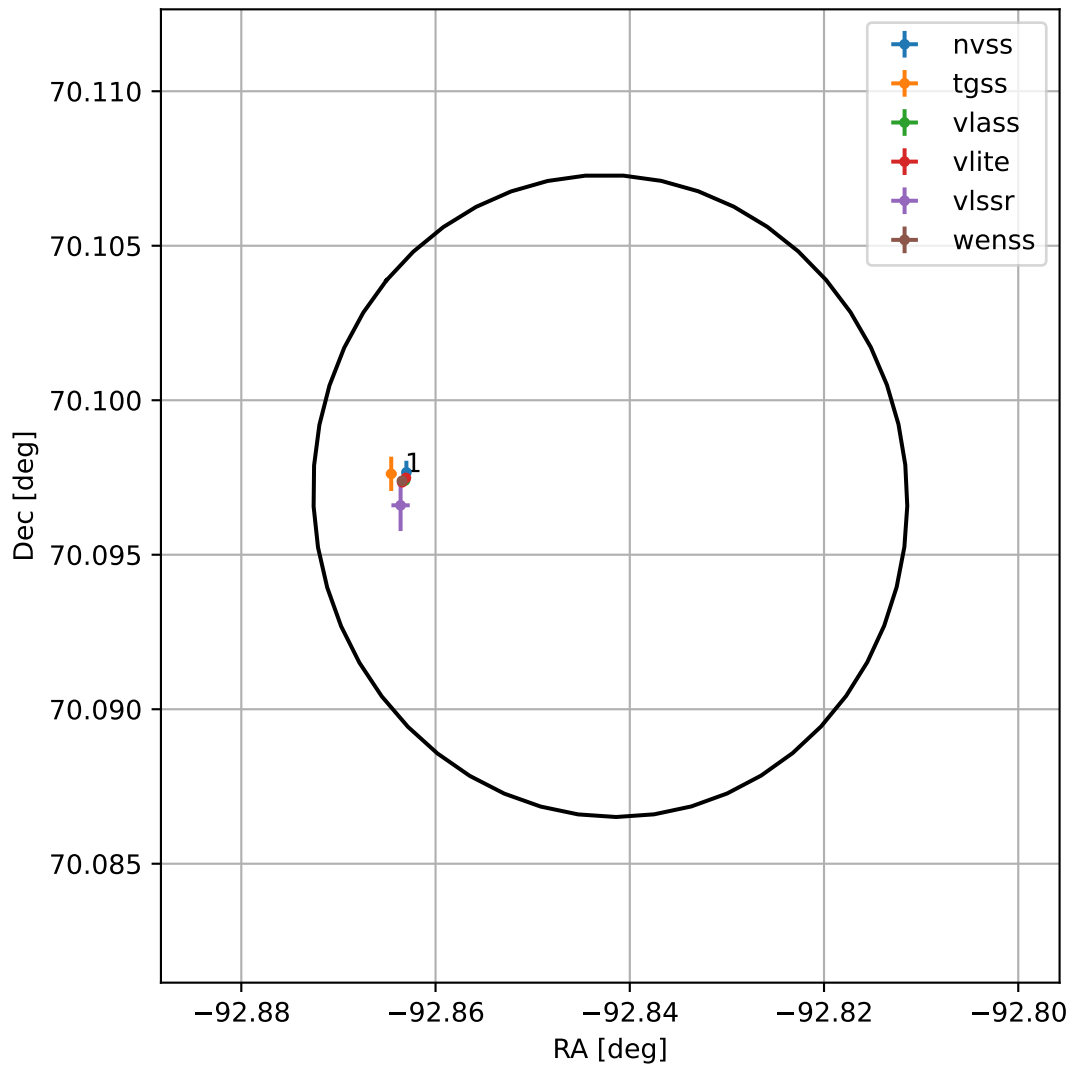
4FGL J1748.6+7005
