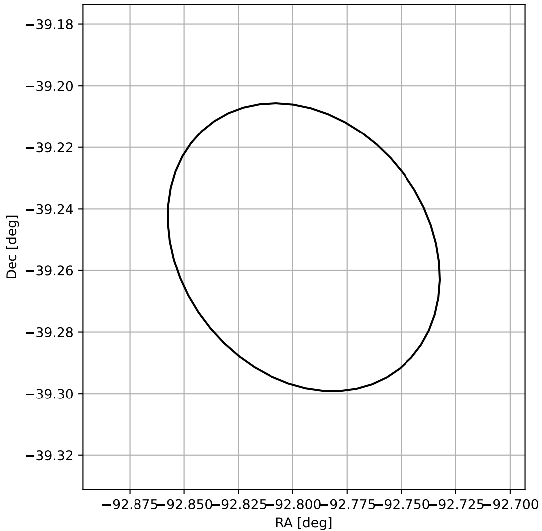
4FGL J1748.8-3915
