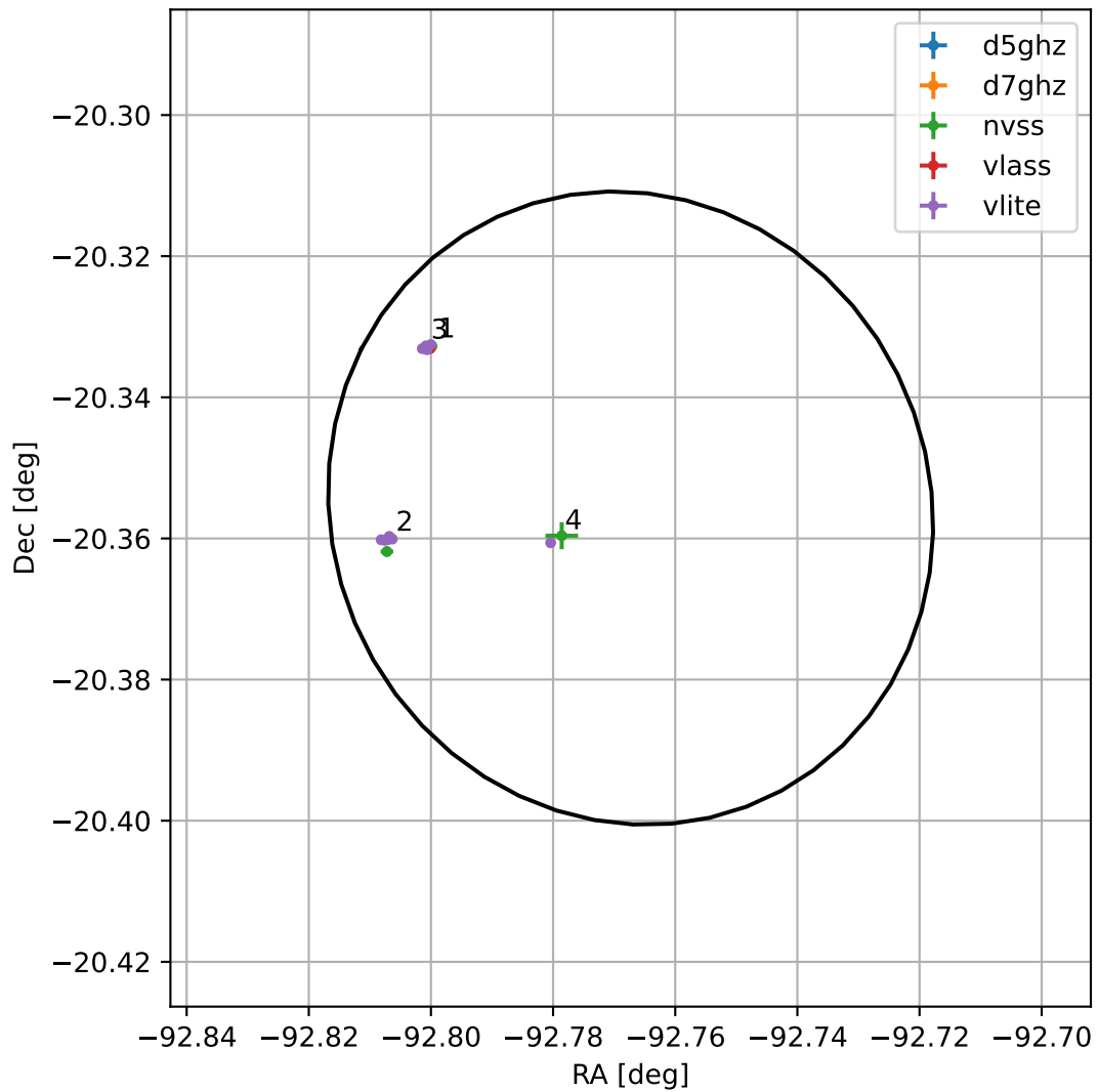
4FGL J1748.9-2021
