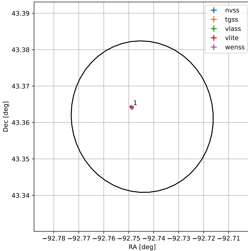
4FGL J1749.0+4321
