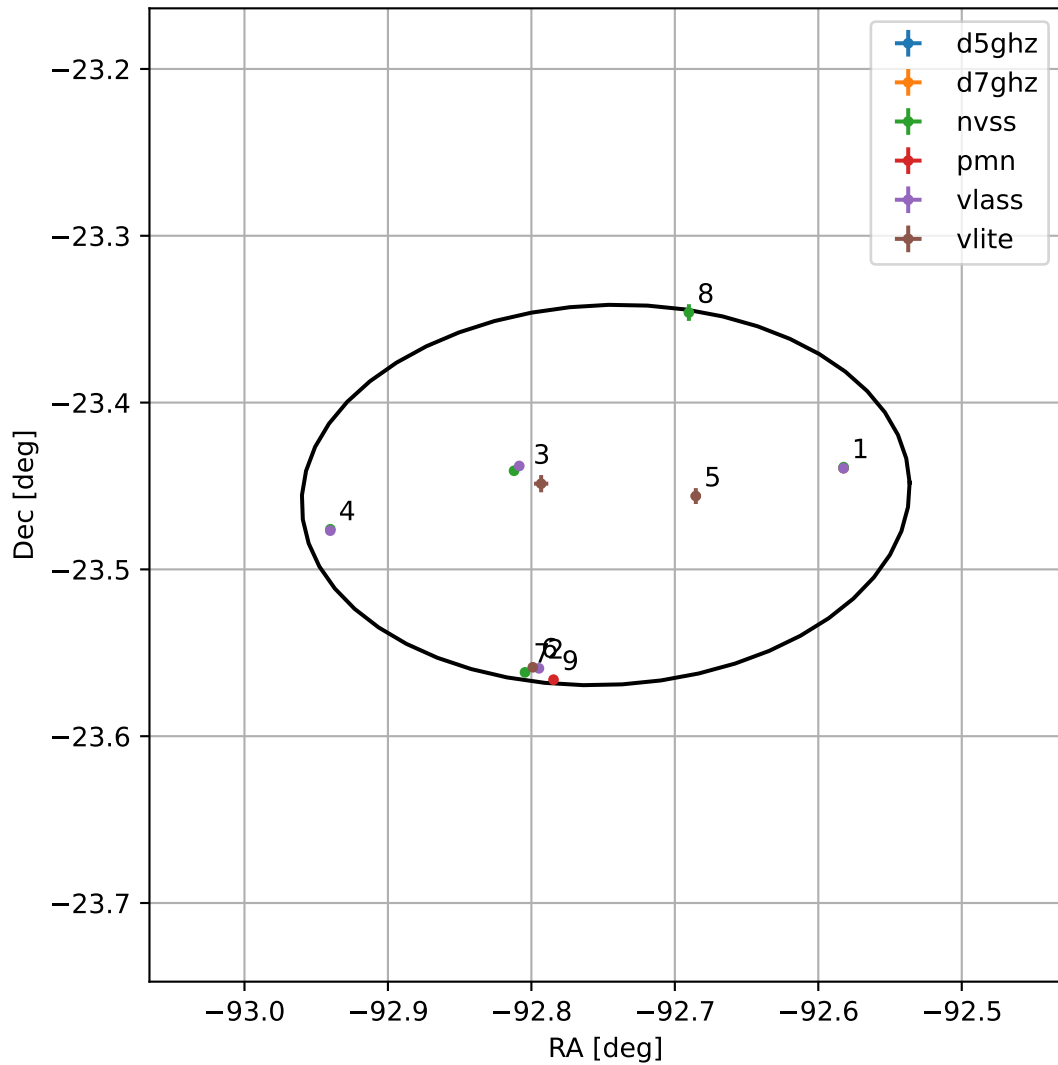
4FGL J1749.0-2327
