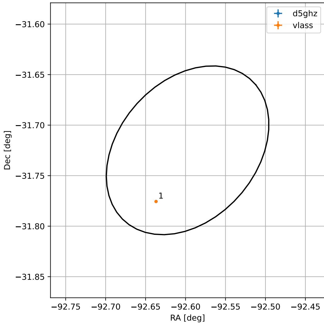
4FGL J1749.6-3143
