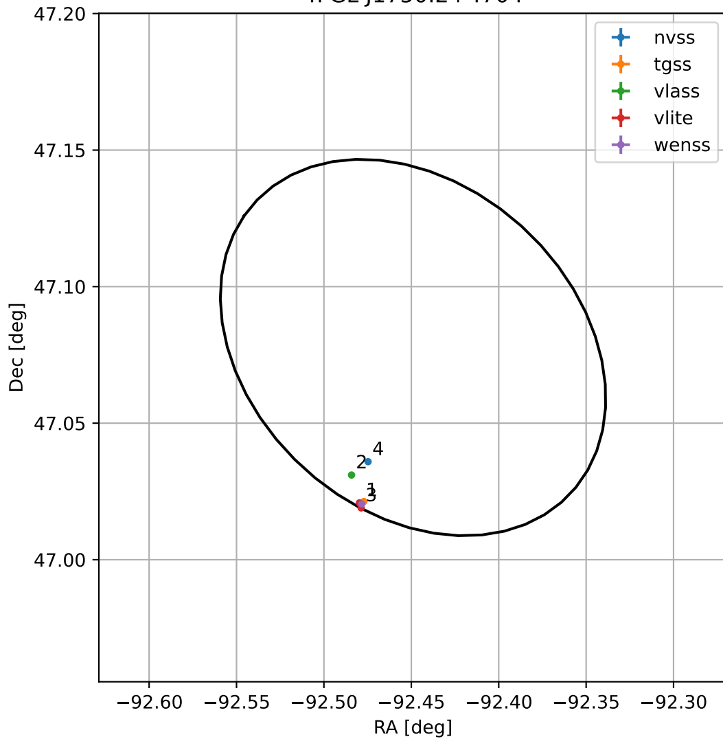
4FGL J1750.2+4704
