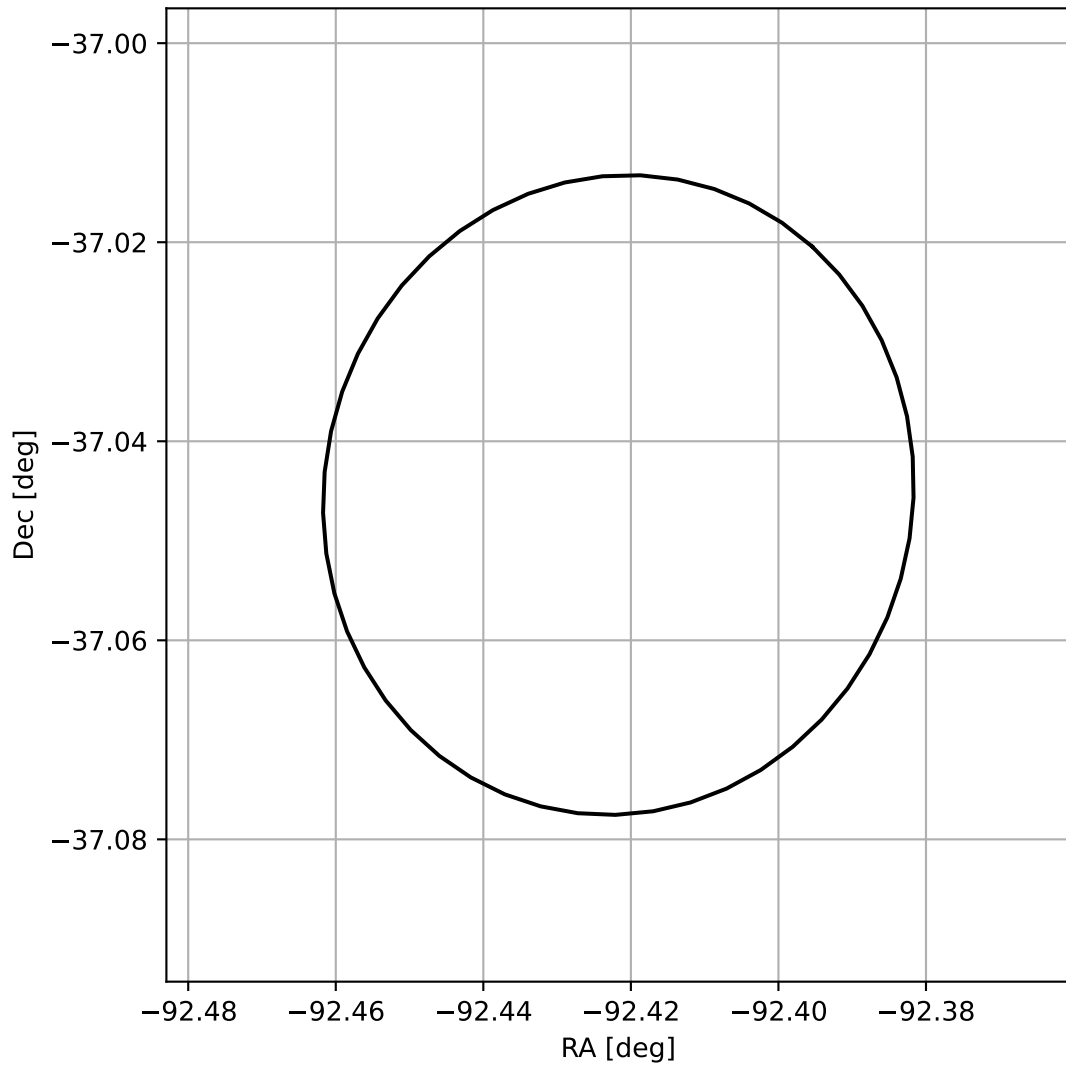
4FGL J1750.3-3702
