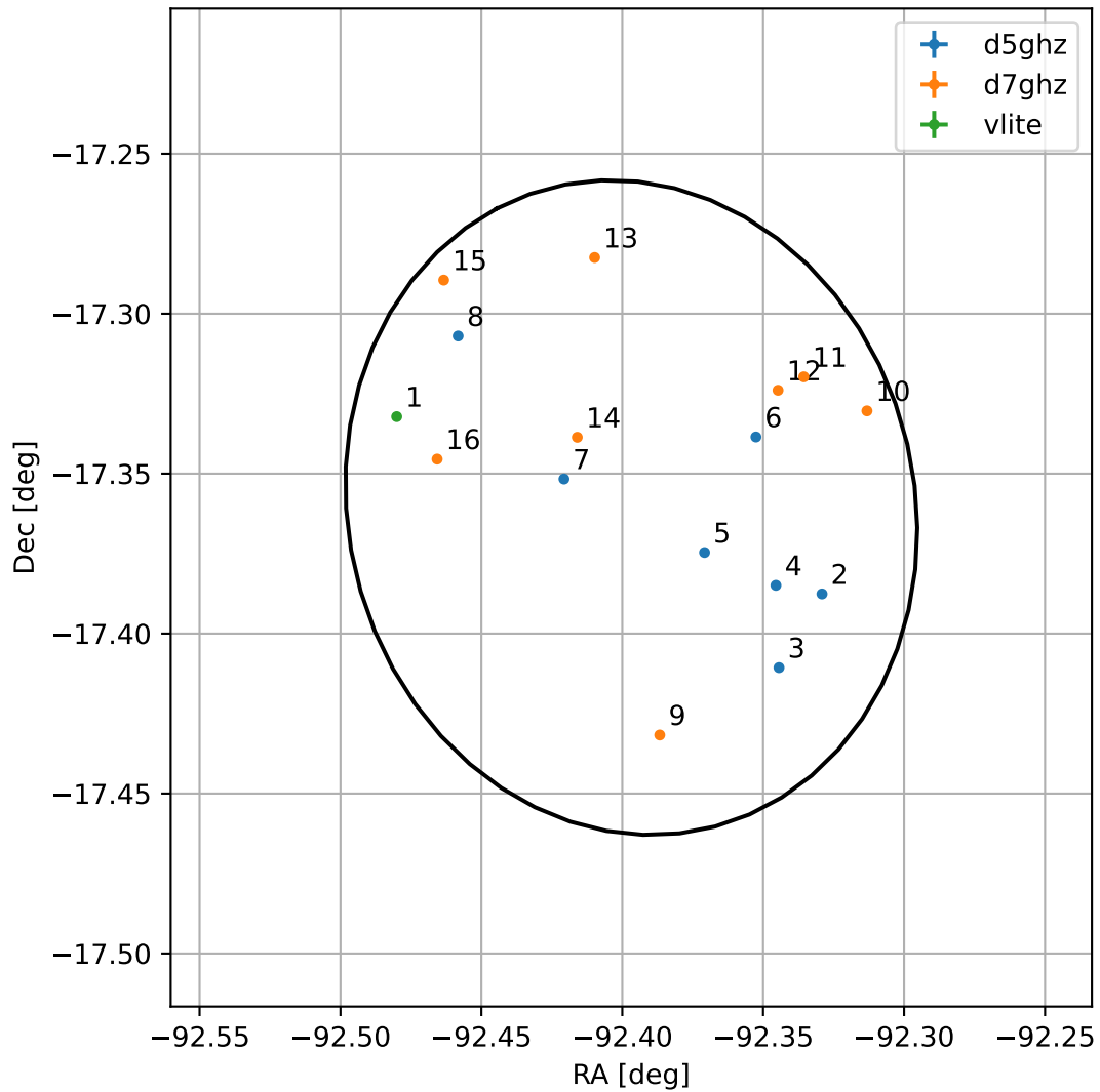
4FGL J1750.4-1721
