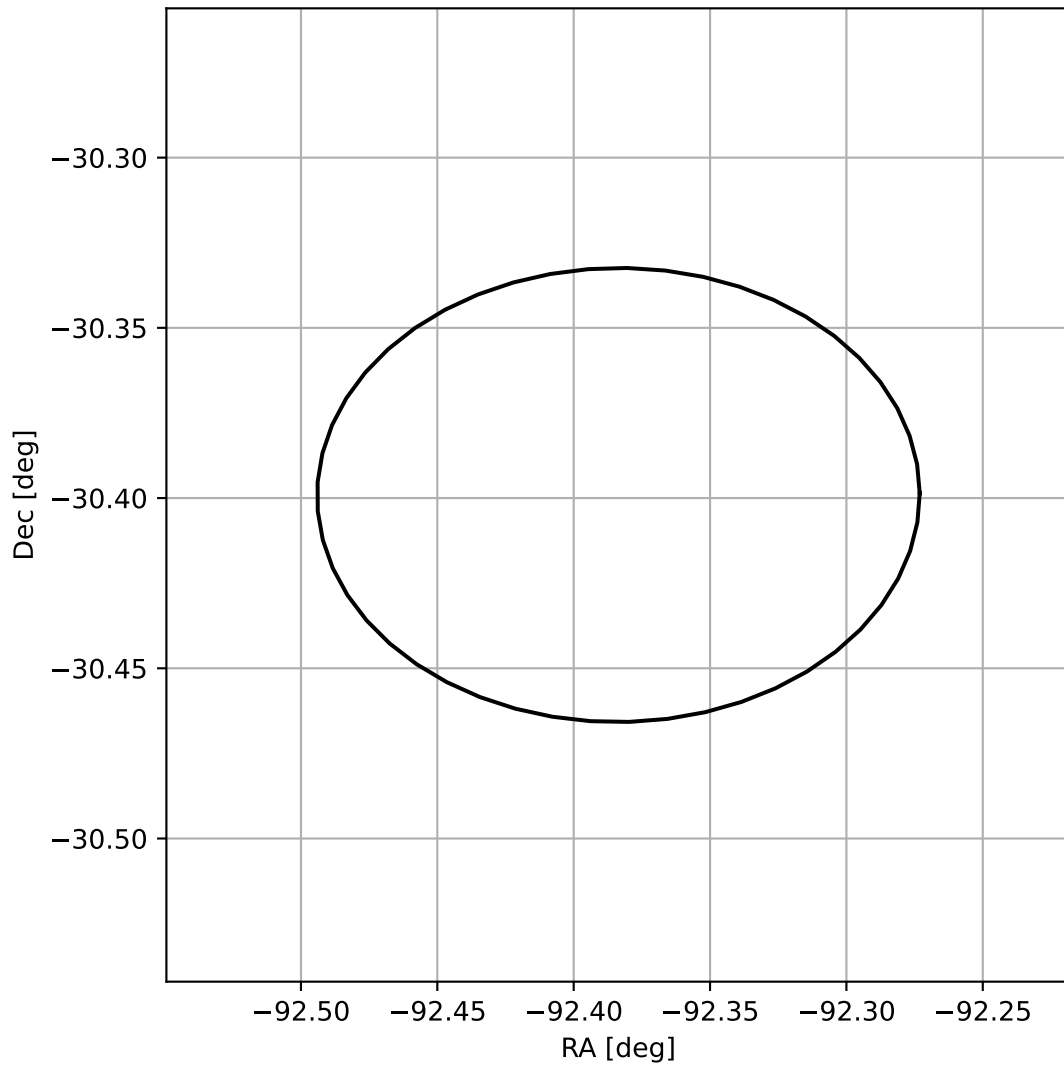
4FGL J1750.4-3023
