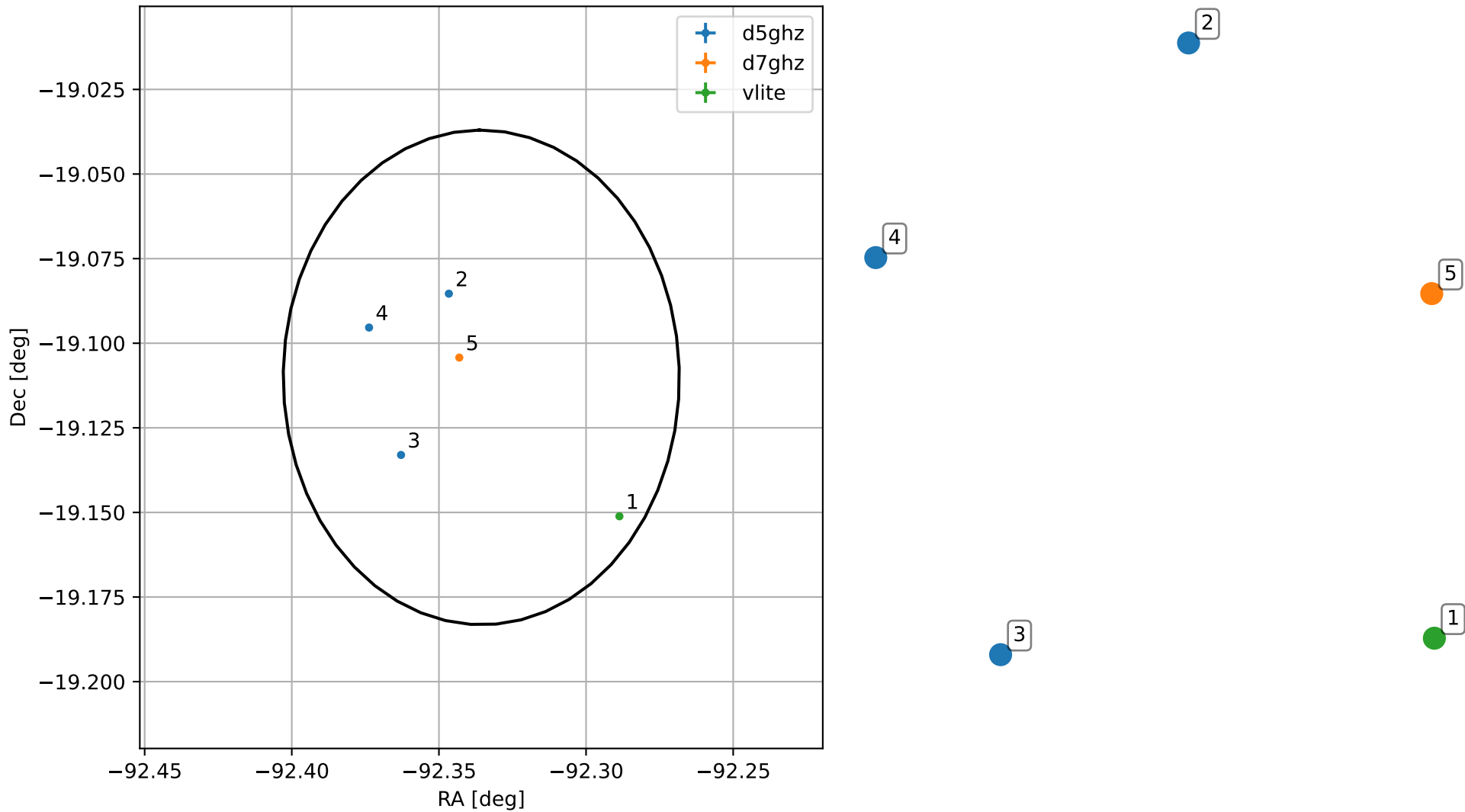
4FGL J1750.6-1906
