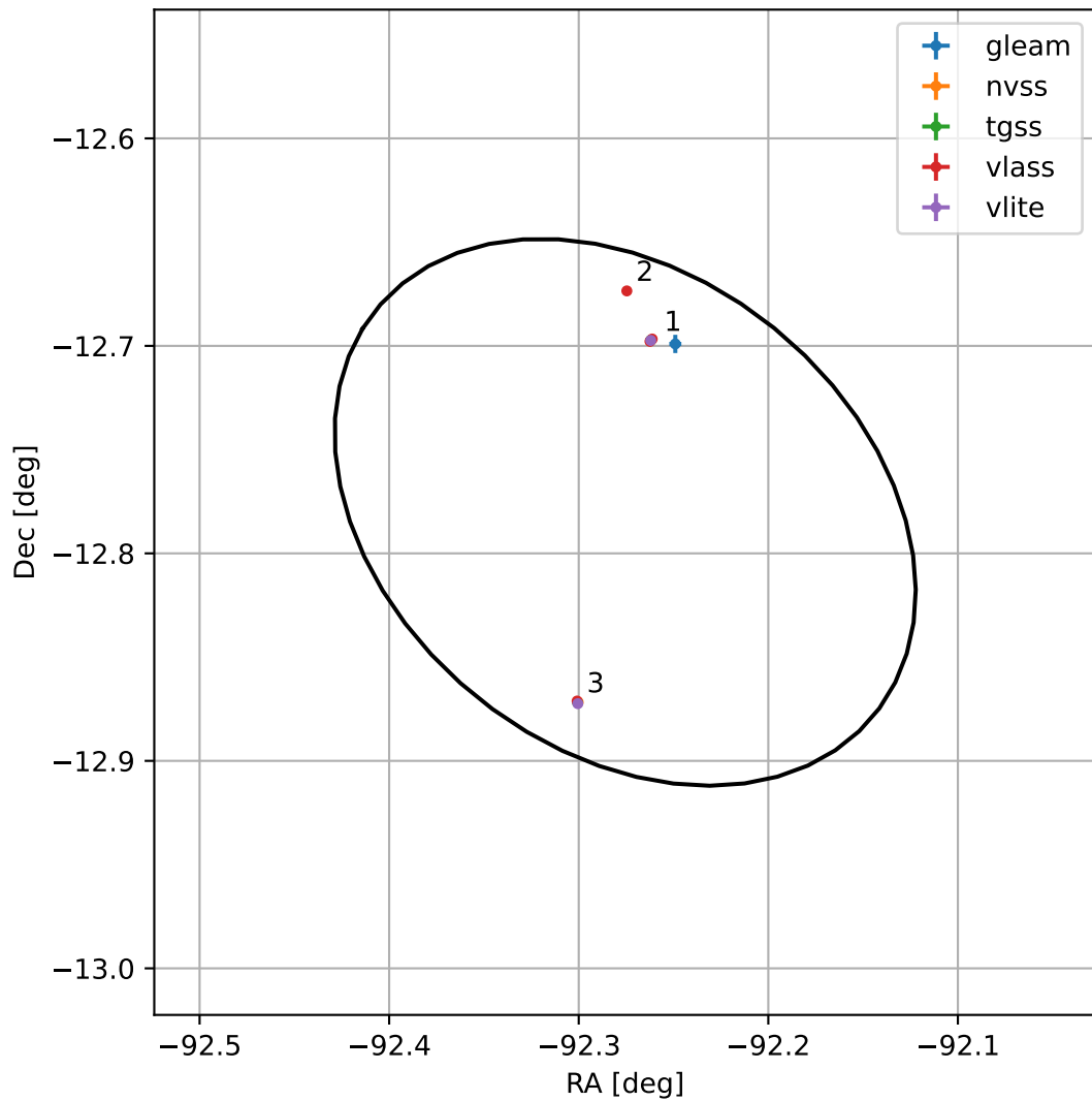
4FGL J1750.8-1246
