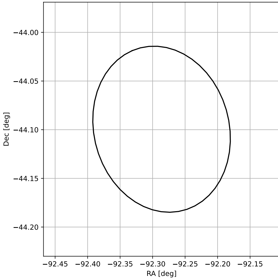
4FGL J1750.8-4405
