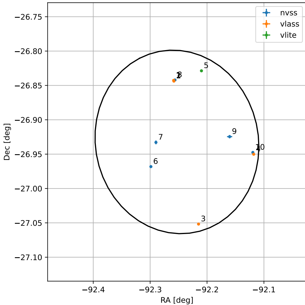
4FGL J1750.9-2655
