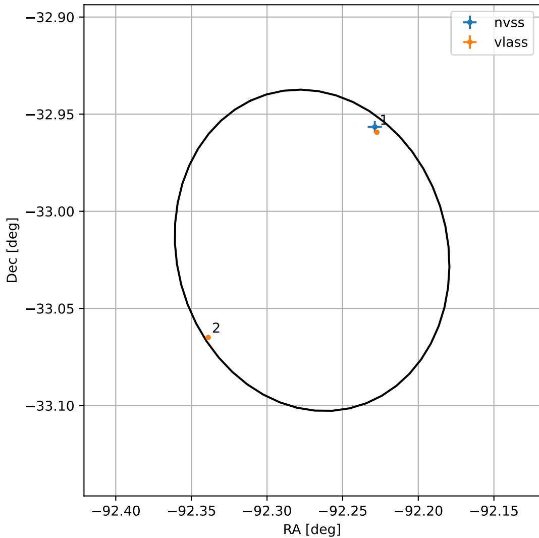
4FGL J1750.9-3301
