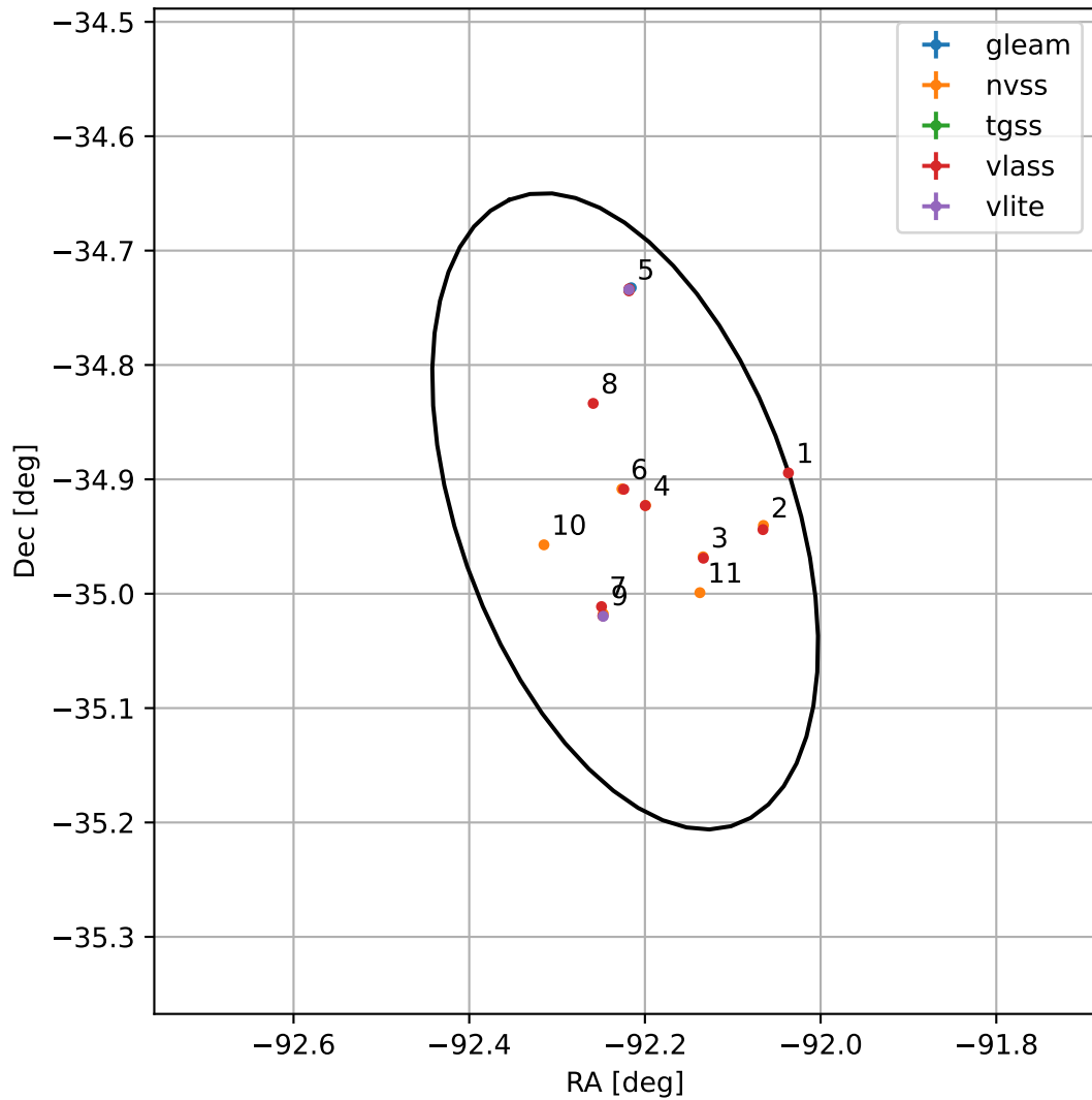
4FGL J1751.1-3455
