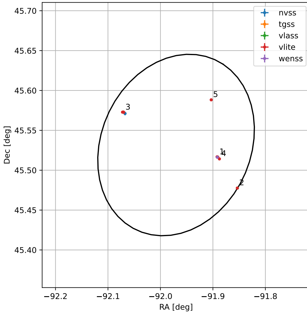
4FGL J1752.1+4531
