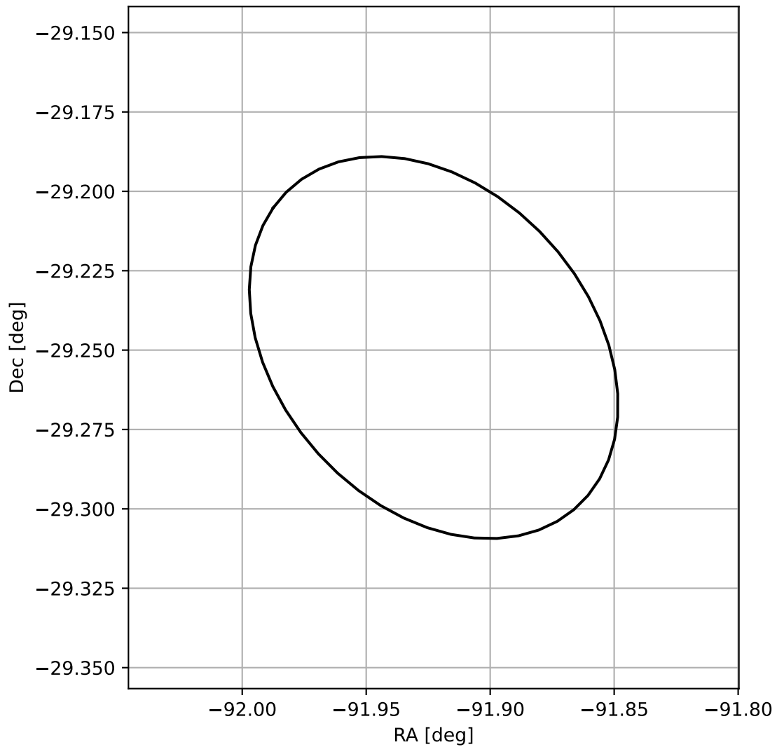
4FGL J1752.3-2914
