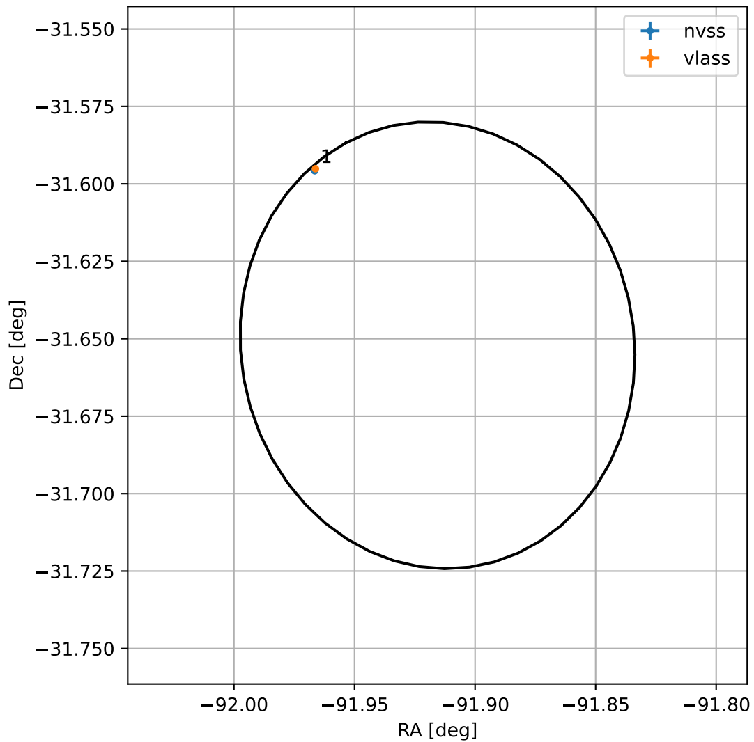
4FGL J1752.3-3139
