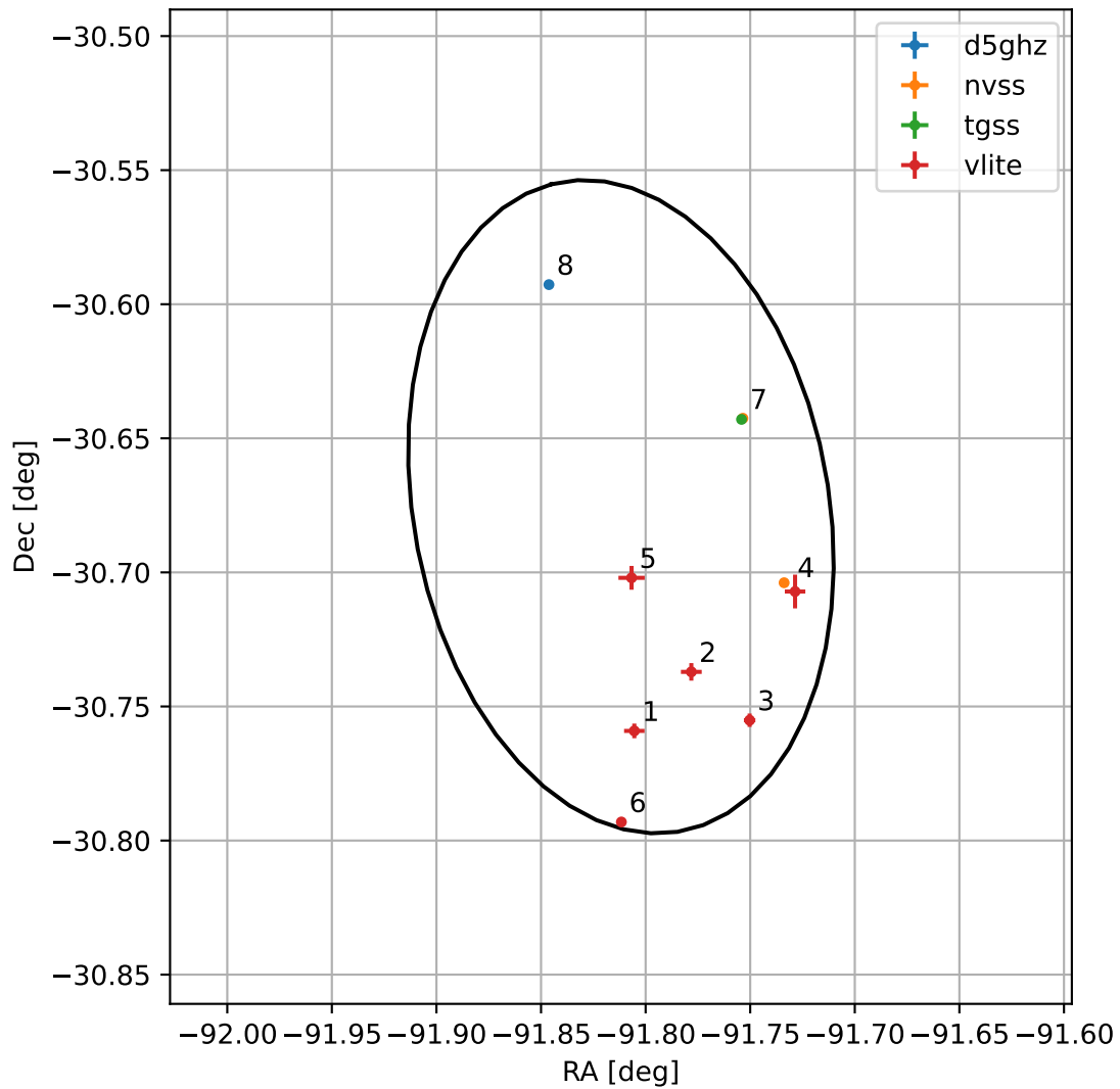
4FGL J1752.7-3040
