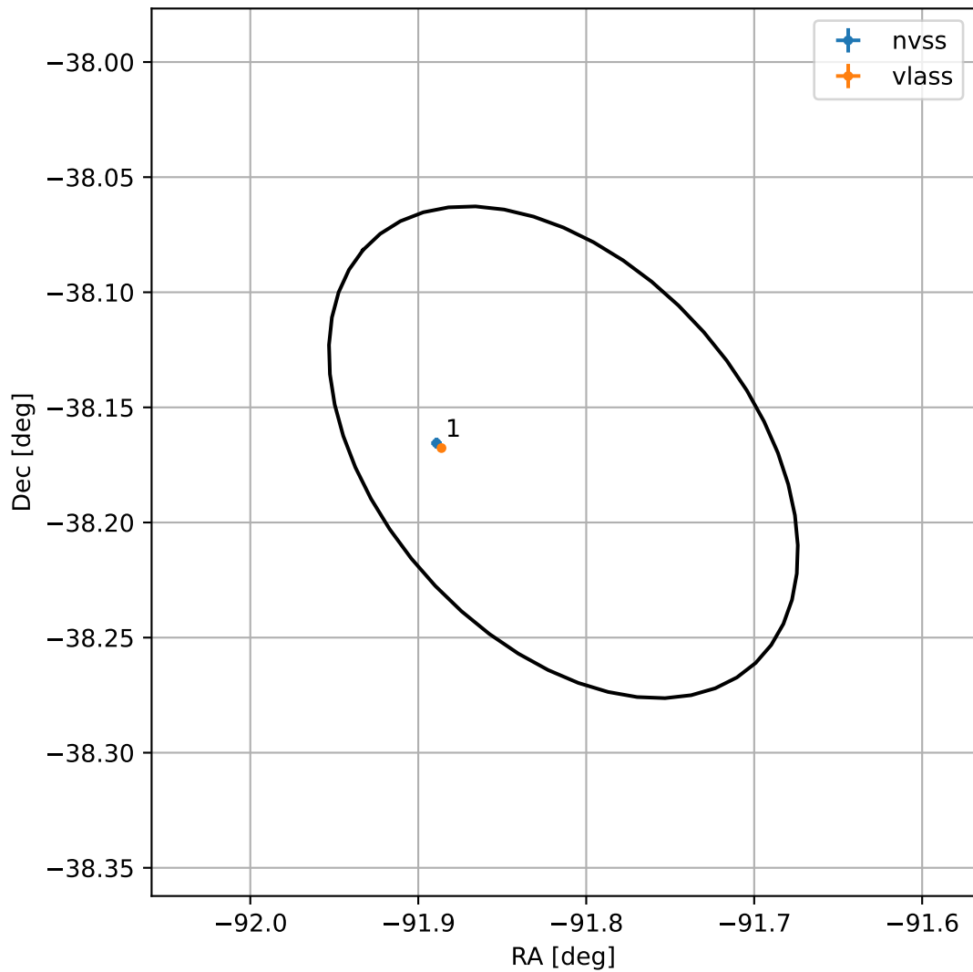
4FGL J1752.7-3810
