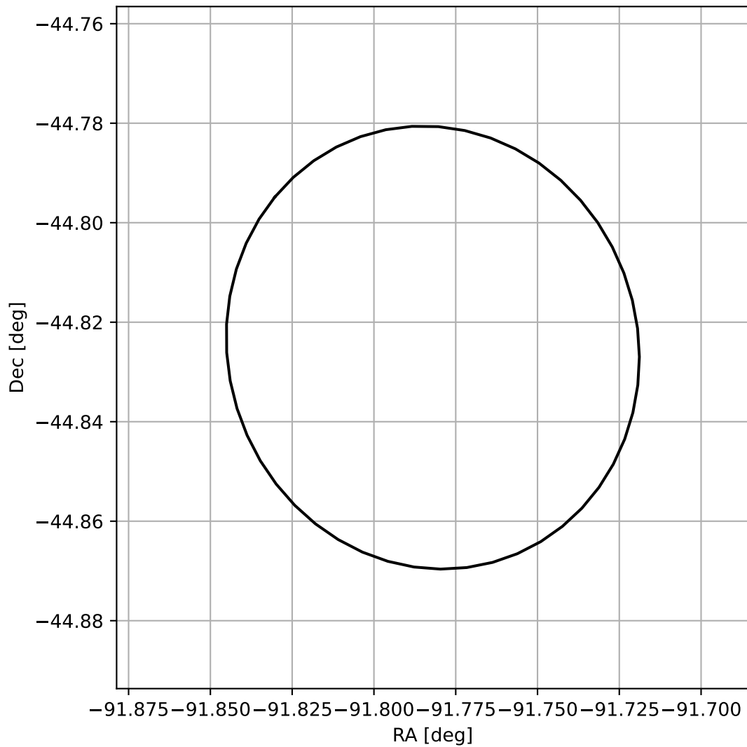
4FGL J1752.8-4449
