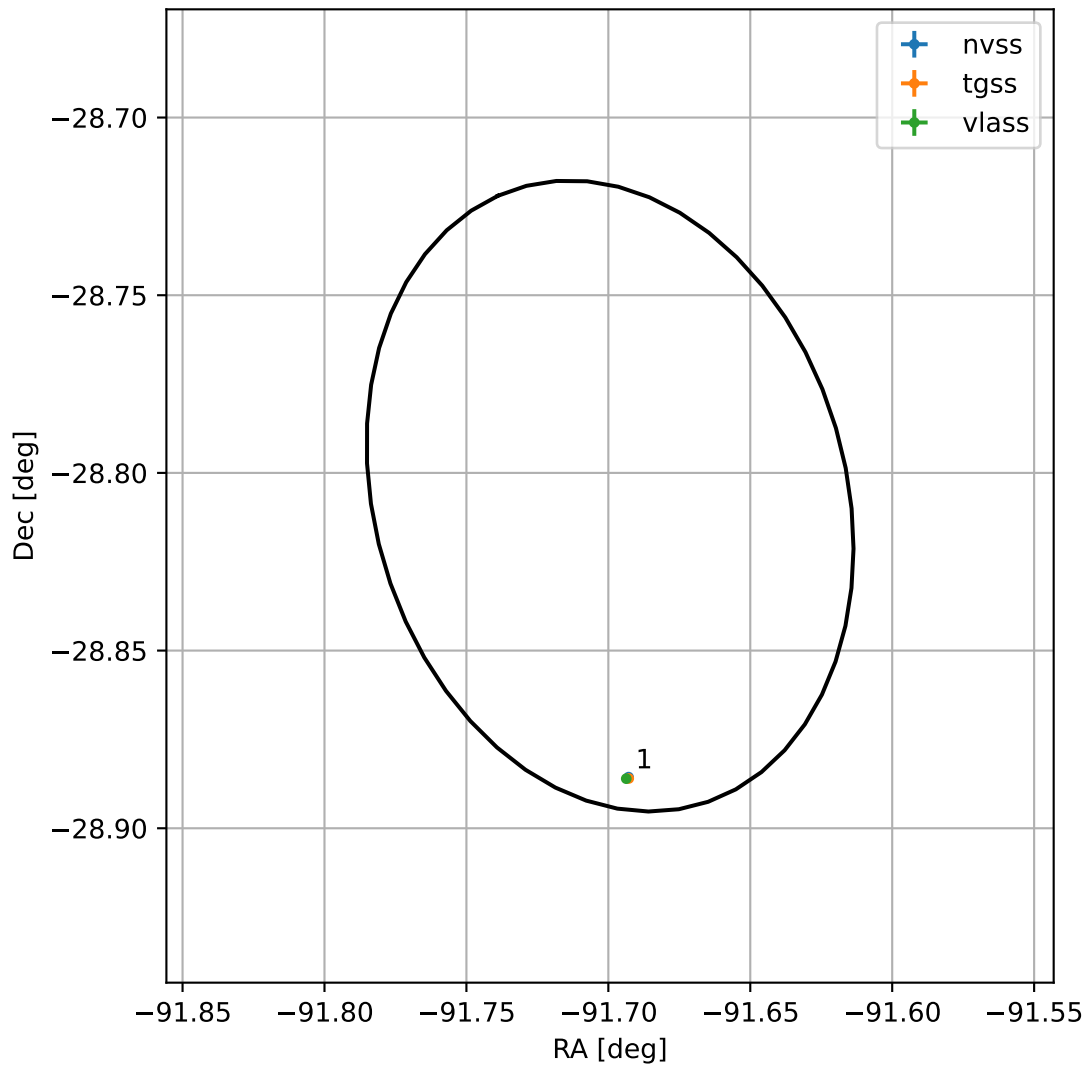
4FGL J1753.2-2848
