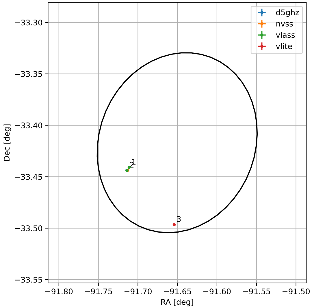
4FGL J1753.3-3325
