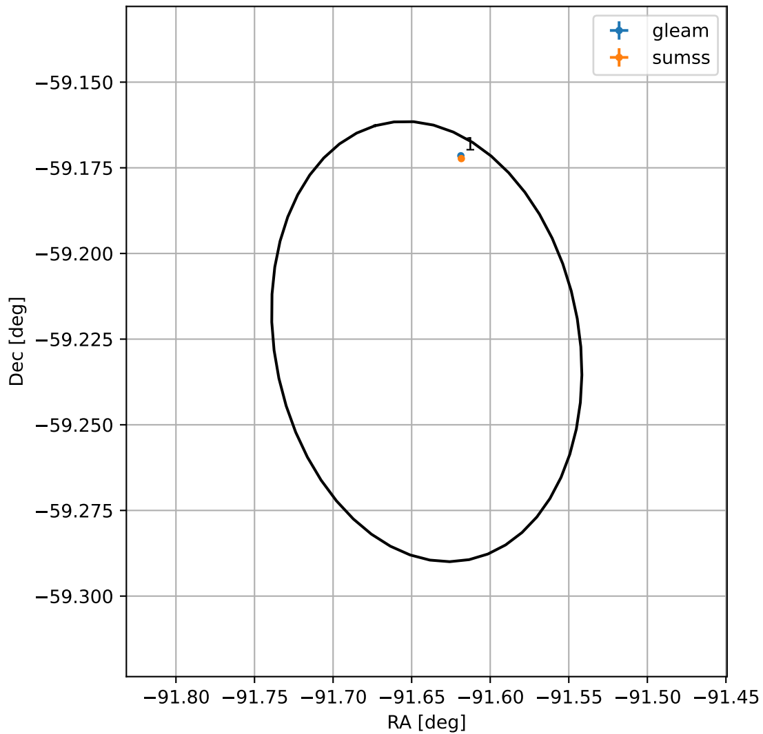
4FGL J1753.4-5913
