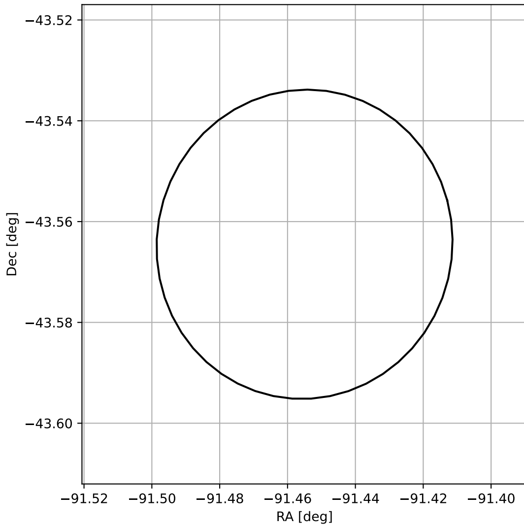
4FGL J1754.1-4333
