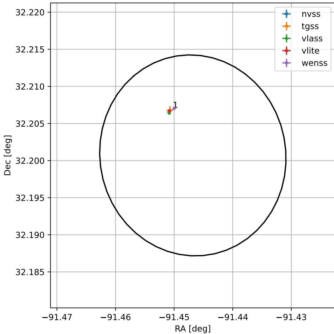
4FGL J1754.2+3212
