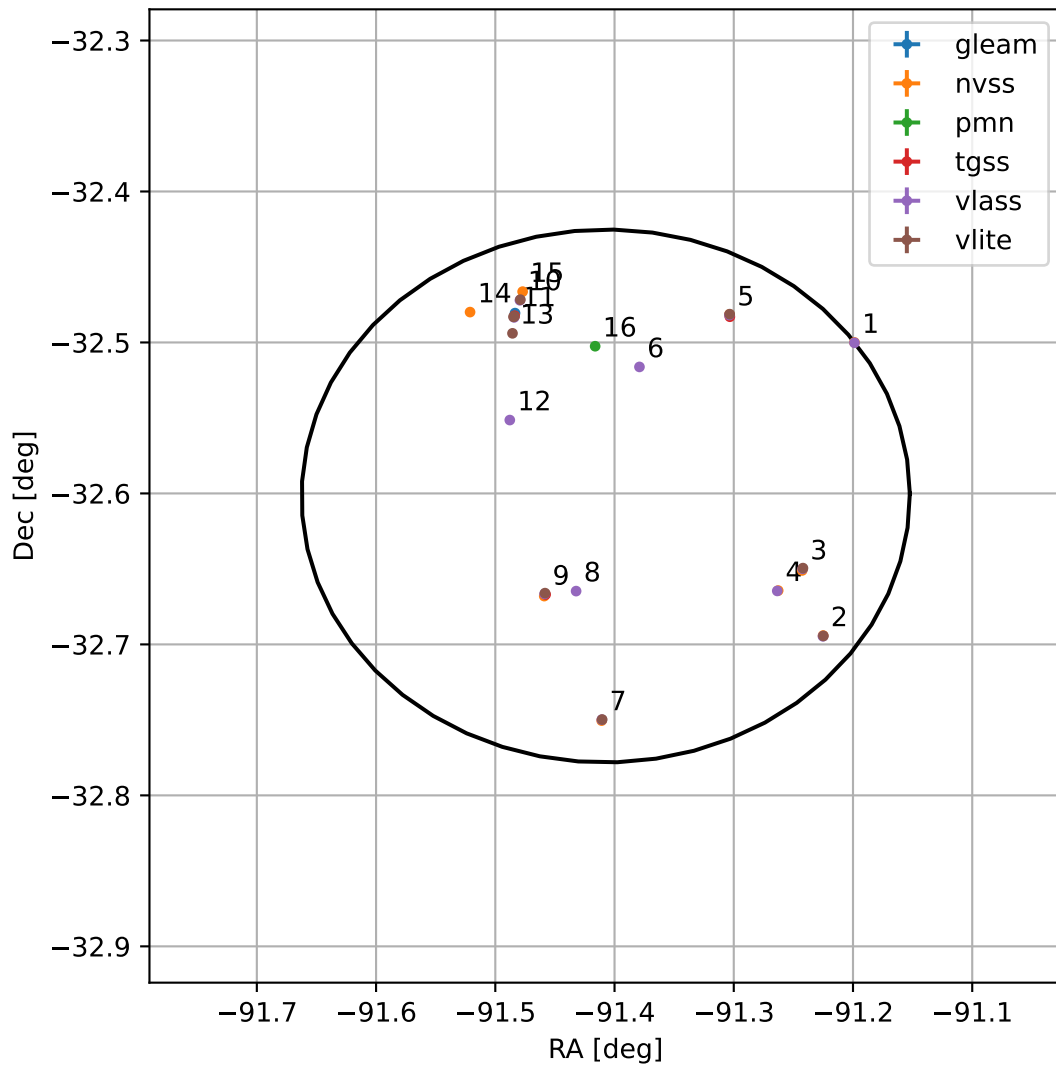
4FGL J1754.3-3236
