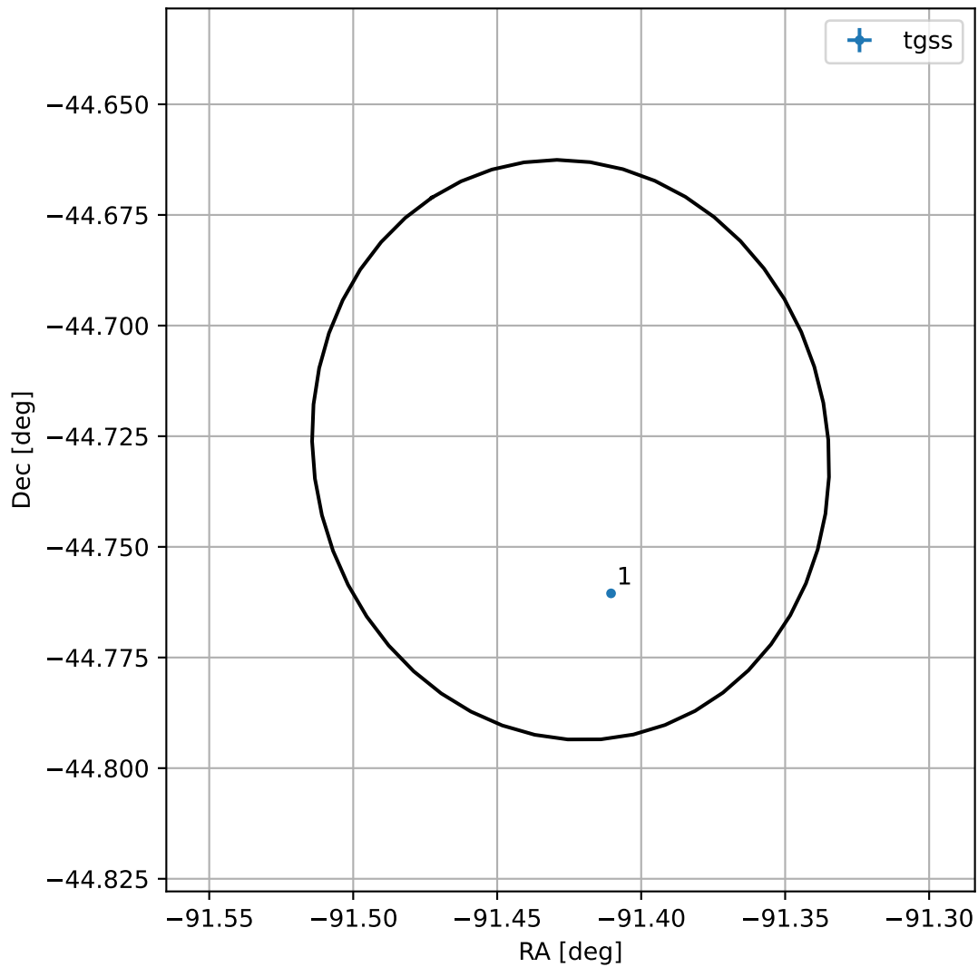
4FGL J1754.3-4443
