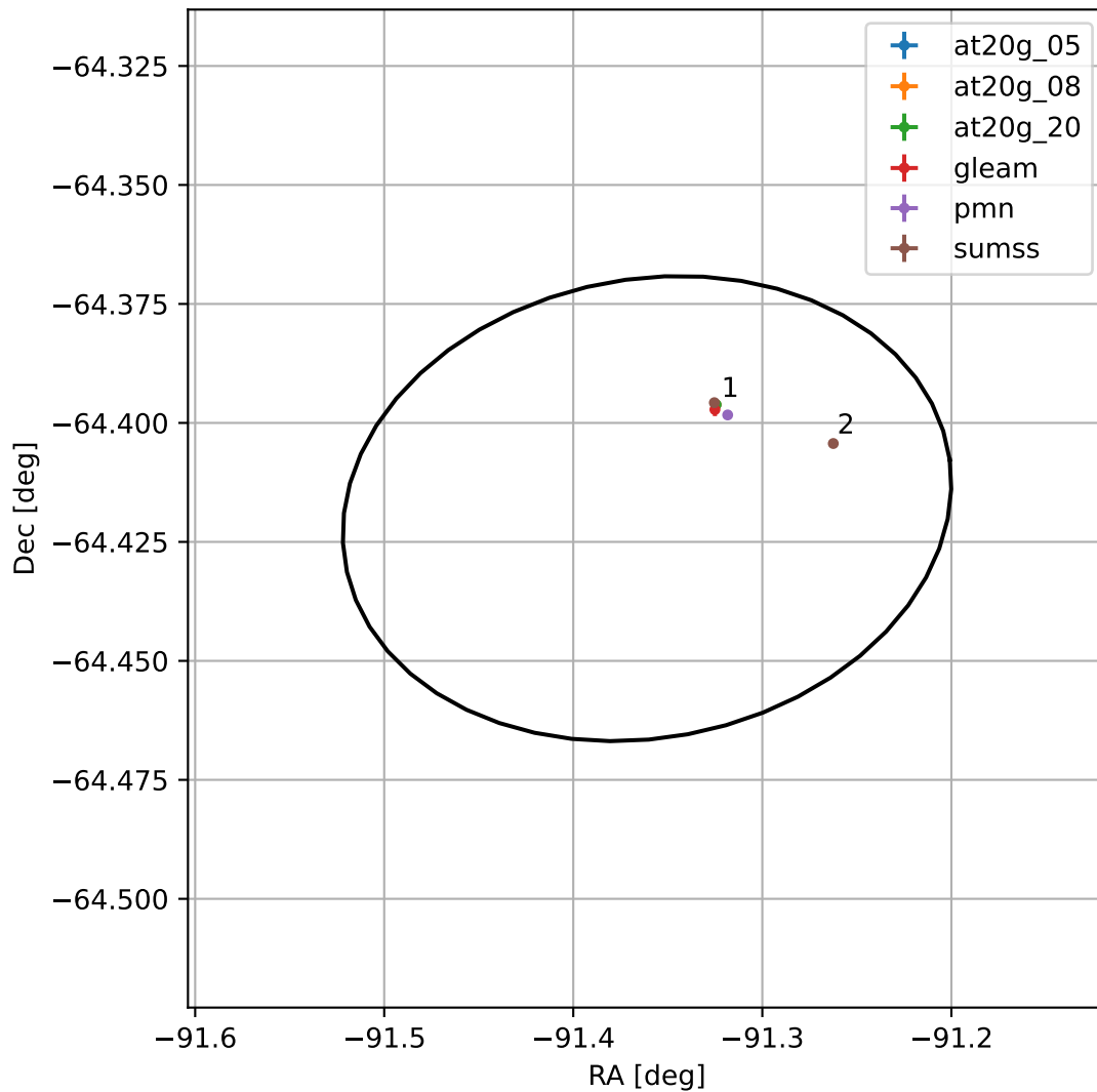
4FGL J1754.5-6425
