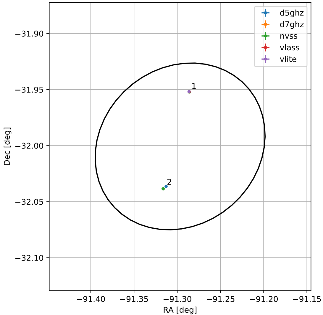
4FGL J1754.8-3200
