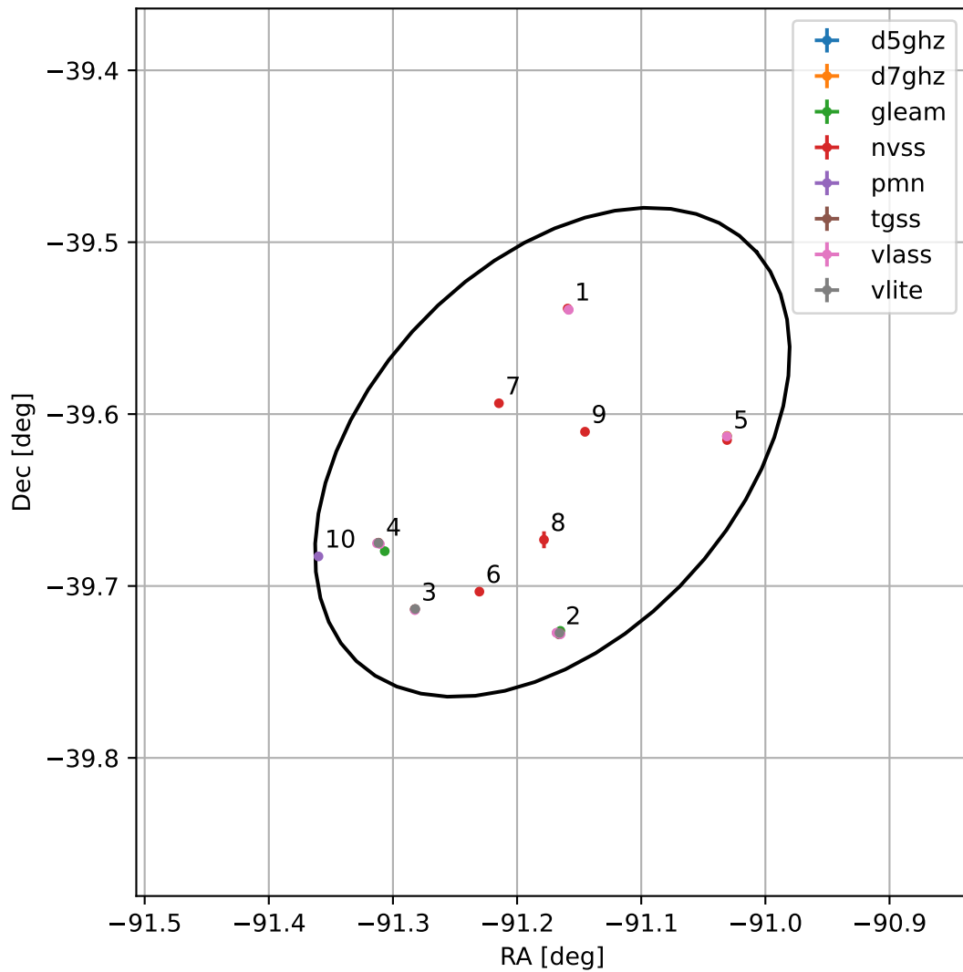
4FGL J1755.3-3937
