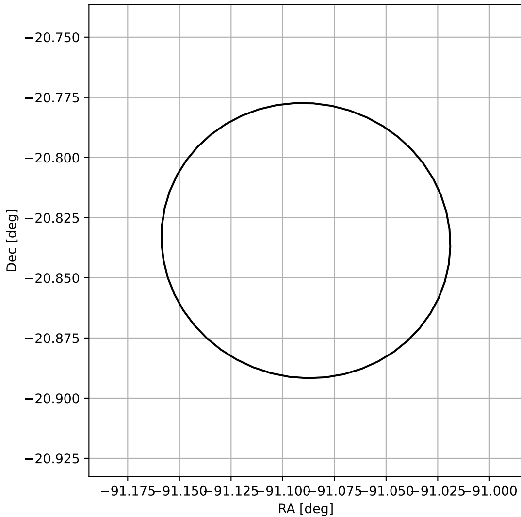
4FGL J1755.6-2050
